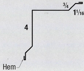
4 - Inside Corner
