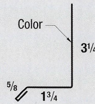
11 - Drip Cap
