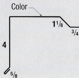
10 - Gable Trim
