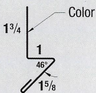
13 - Rat Guard
