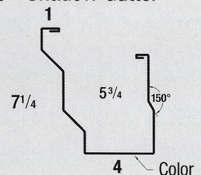
16 - Shadow Gutter
