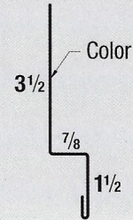
14 - Wainscot Trim
