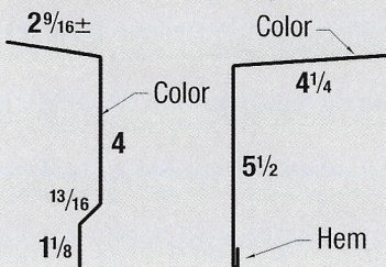
6 - Fascia Simple Eave
