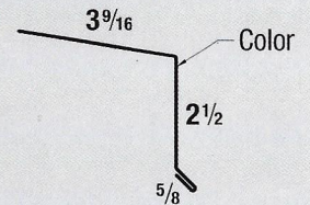
8 - Eave Drip Trim
