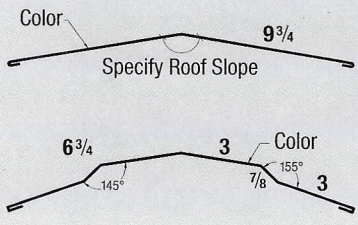
3 - Rake & Corner
